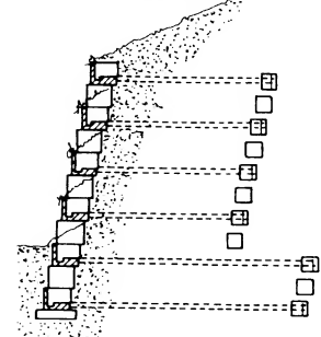
15 Wall with land anchors (Lüdenschied example)
